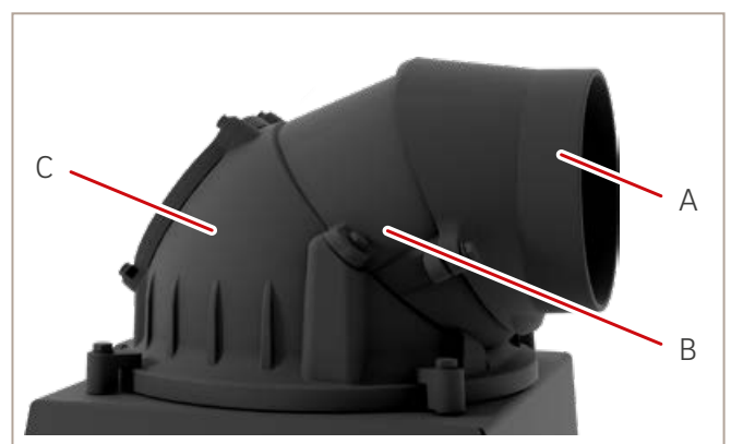
Abb. 7: Gusskuppel, Position 90°
